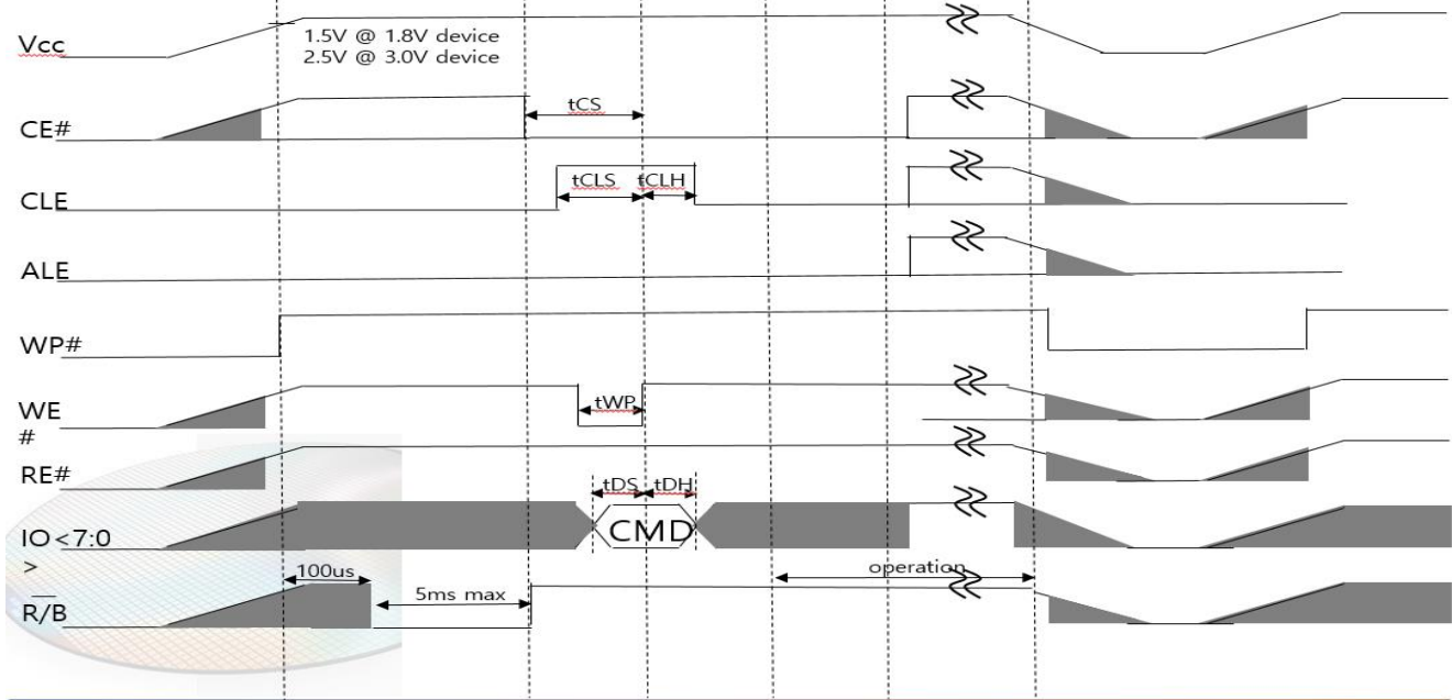
Figure 31 : Power up time sequence
