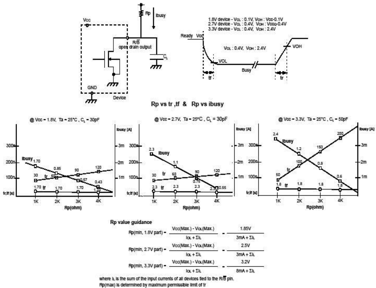
Figure 32 : Ready/Busy Pin electrical application
